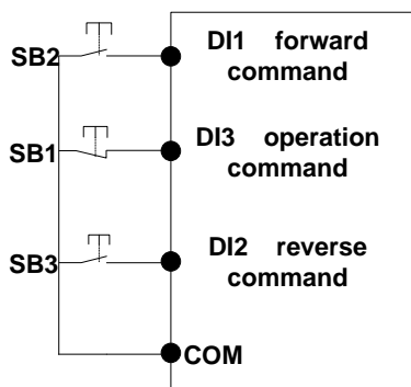
Figure 3: Three-line mode1
