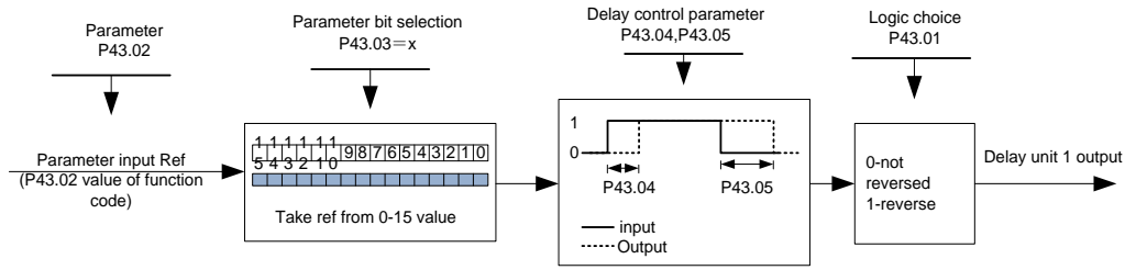
Delay unit 1 block diagram
