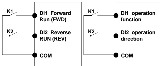
Figure1: Two-line mode 1
