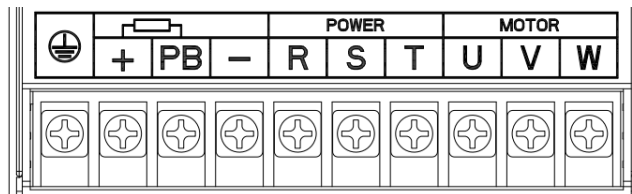
Figure 3-6 SIEZ main circuit terminal diagram
