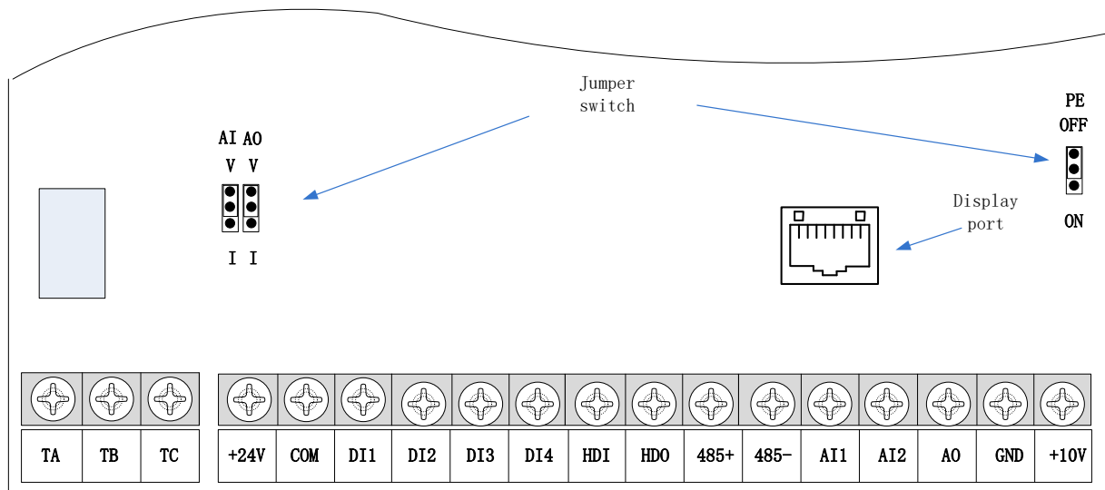
Figure 3-6 Schematic diagram of the VFD510 control circuit terminal (SIZE A/B)
