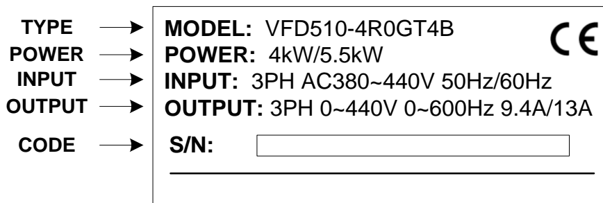
2-1 name plate
