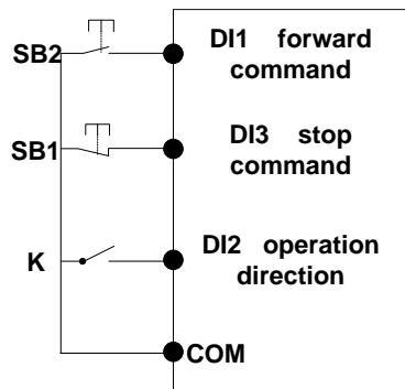
Figure 4: Three-line mode2
