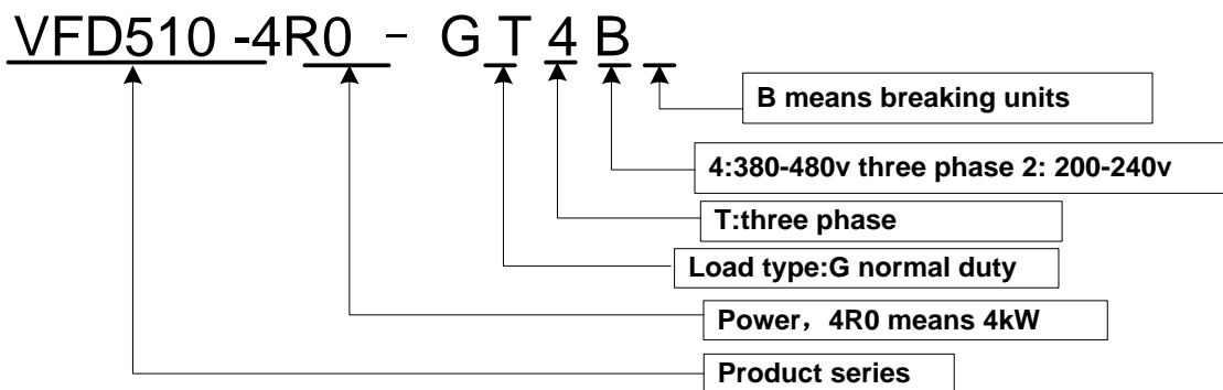
2-2 model instruction
