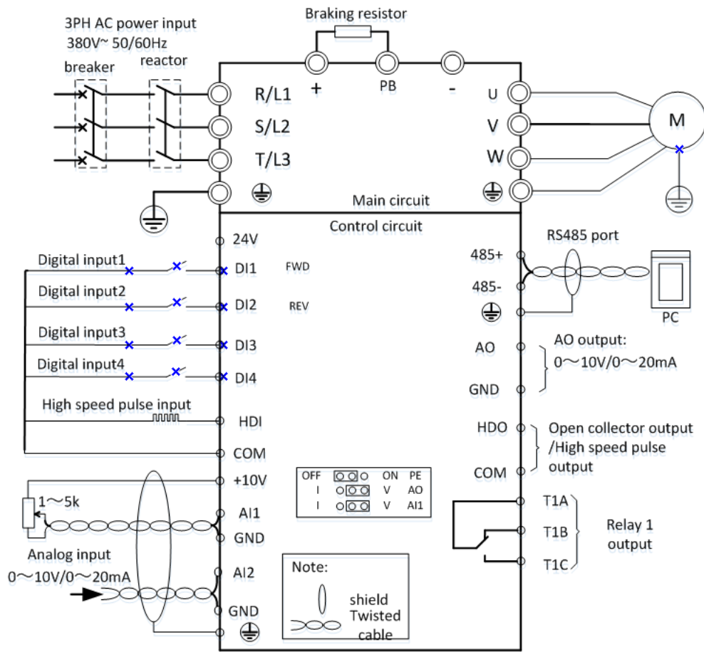
Figure 3-3 (SIZE A/B) standard wiring diagram
